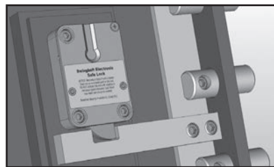
SWING BOLT LOCK
