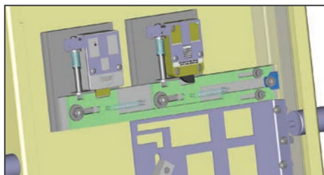
Safe locked shut – Both locks engaged, bolts extended
