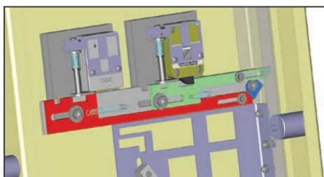
Safe open – Lock on the left unlocked, lock on the right locked, bolts retracted
